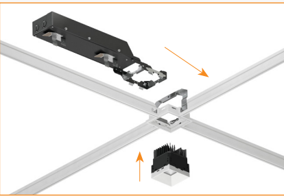
2. USAI Connect housing snaps on to tee grid and yoke from above. Install light from below. Make electrical connection with quick connects.
