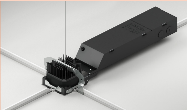
Shown with hanger wire Each USAI® Connect™ LED light fixture is shipped complete with everything needed to install. No tools are required.
