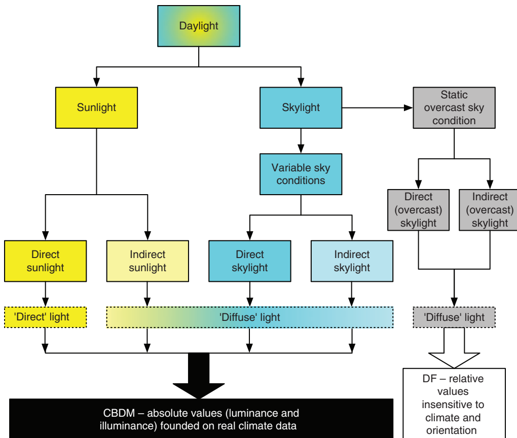
Figure A1 The components of daylight and their relation to the DF and climate-based modelling approaches
